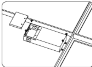
■ Driver mounting
